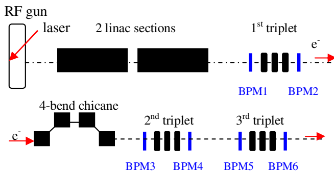
FIG. 1. (Color) Schematic layout of the ATF H-line; the beam bends in the vertical ( y ) plane in the chicane.
